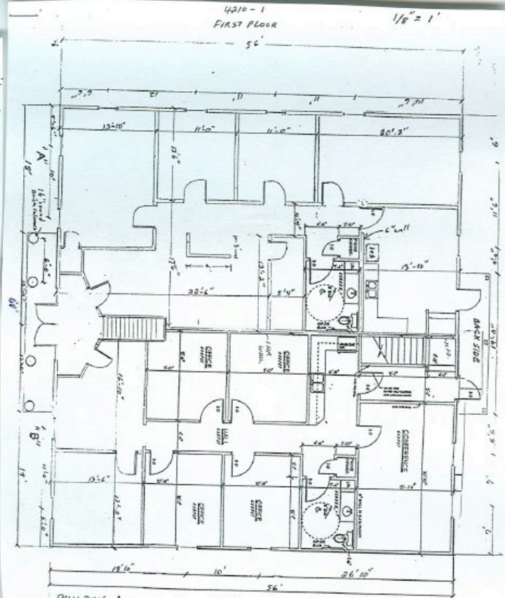
BUILDING 1 FIRST FLOOR 3416 SF
